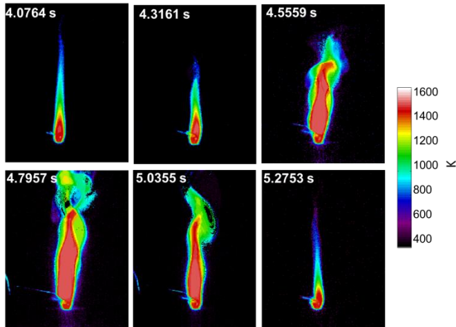
Figure 6 Temperature profile of the plume during the explosion generated by the burning of black powder.
