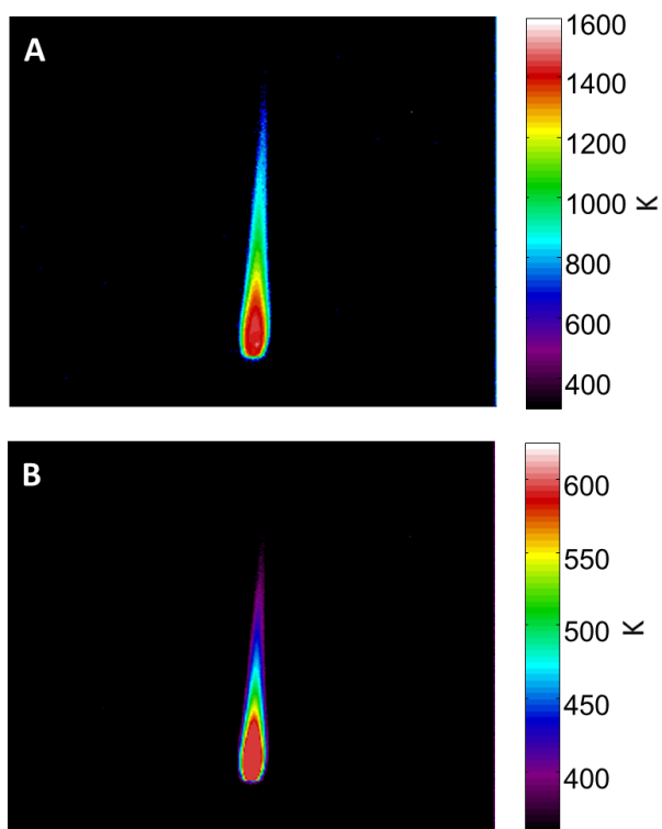
Figure 5 A) Estimated temperature profile of carbon dioxide in the flame obtained by the optimization and B) Temperature profile of the candle's plume obtained by broadband imaging (filter #1).
