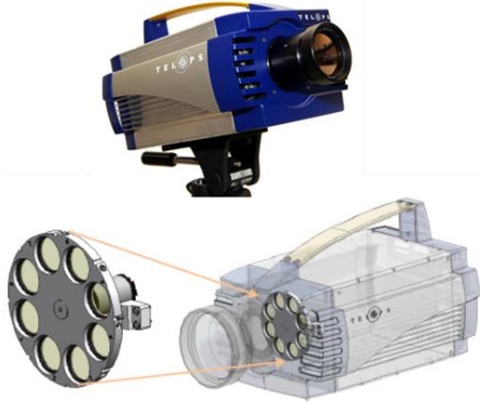
Figure 1 The Telops MS-IR camera and the filter wheel system.
