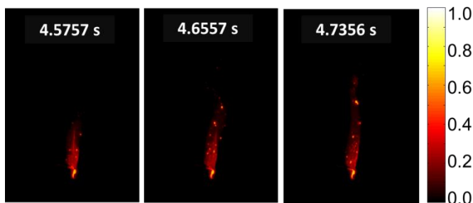
Figure 7 Carbon soot seen using the "through flame" filter (filter #3) for 3 consecutive wheel turns.
