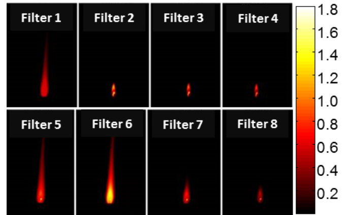
Figure 3 Relative individual spectral channel responses during candle's combustion.
